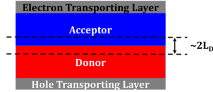
Fig. 3. 4. Structure of a bilayer device. Only the excitons which are generated within the diffusion length of the D/A interface (between the dashed lines) dissociate and give rise to free charge carrier.
