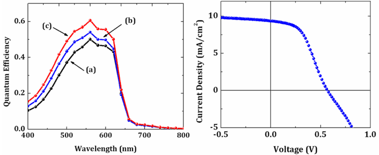
Fig. 5. 7. Left–QE of hybrid P3HT:PCBM cells for different CH_4 flow during growth of ETL in PECVD reactor: (a) 0, (b) 3, and (c) 6 sccm. Right–With 6 sccm CH_4 flowing during ETL growth a barrier emerges in the JV characteristic.
