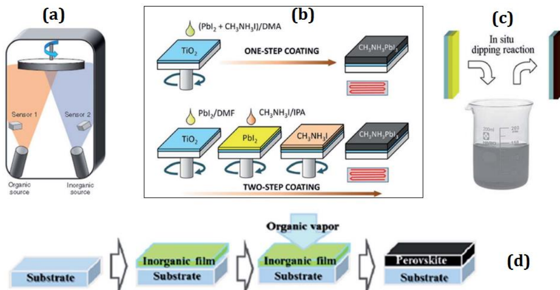
Fig. 6.11. Methods for synthesizing perovskite thin films for solar cells: (a) Dual-source evaporation, (b) one-step (top) and two-step (bottom) spin-coating, (c) in-situ dipping, and (d) vapor-assisted deposition.
