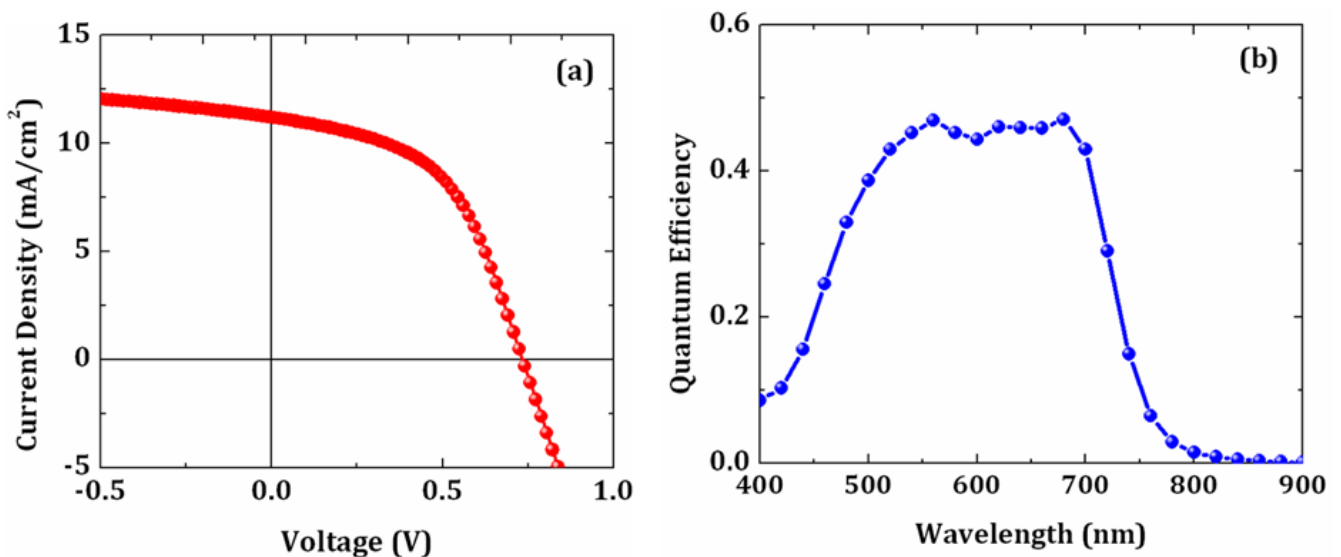
Fig. 5. 8. (a) JV characteristics, and (b) QE of a PTB7:PCBM 70 hybrid cell with a-(Si,C):H ETL. The optimized performance was obtained for 6 sccm of CH_4 flow during ETL growth.
