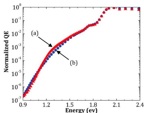
FIG. 6. Subgap quantum efficiency data for cells deposited on a -(Si,C) (curve a) and a normal P3HT/PCBM cell deposited on PEDOT:PSS (curve b). The results are very similar, indicating similar material properties.
