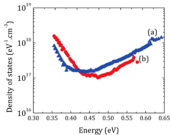
FIG. 5. Density of states at the interface between P3HT and PCBM measured using capacitance-frequency techniques for the two cells, one deposited on \text{Cs}_2\text{CO}_3 (curve b) and one on a\text{-Si} (curve a). The results are very similar.
