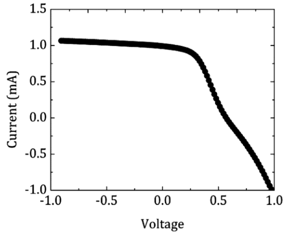
FIG. 4. Illuminated I-V curve when the cell is deposited on a doped a\text{-Si,C} layer. A slight non-ohmic behavior is evident, probably related to the difficulty of doping a\text{-Si,C} as methane content of a\text{-Si,C:H} increases.
