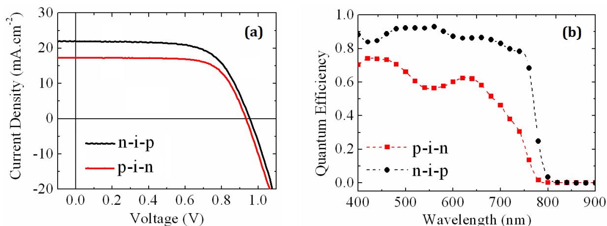
Fig. 6. 16. IV characteristics (a), and QE spectra (b) of n-i-p (black) and p-i-n (red) CH 3 NH 3 PbI 3 solar cells.
