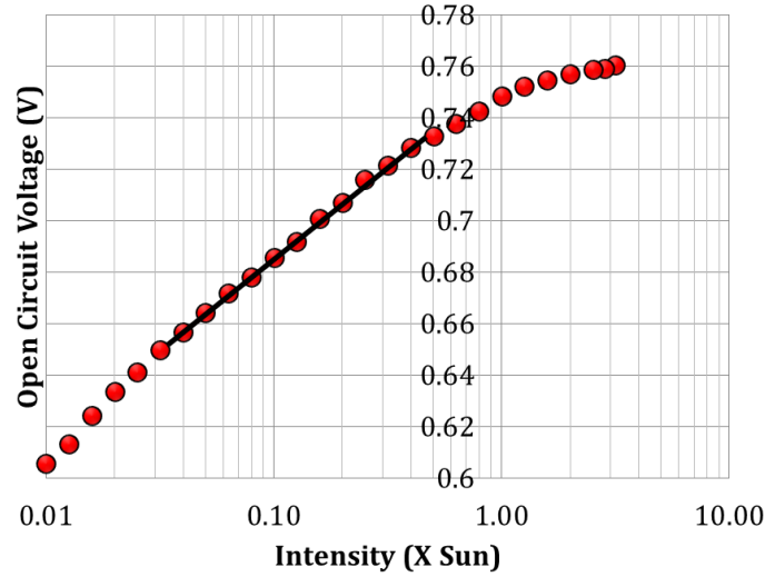
Fig. 4.13. V_{oc} vs. light intensity of a standard PTB7:PCBM 70 cell. The light ideality factor is extracted from the linear region and is about \sim 1.1-1.2 .
