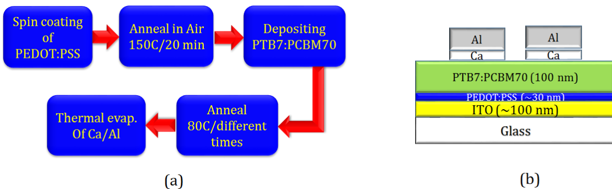
Fig. 4.3. Fabrication process (a), and device structure (b) of a standard p-i-n PTB7:PCBM 70 cell.
