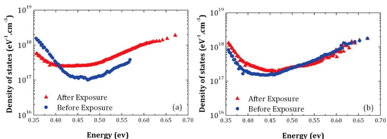
FIG. 8. Changes in defect density before and after exposure for cells deposited on Cs 2 CO 3 (panel a) and on a-(Si,C) (panel b).
