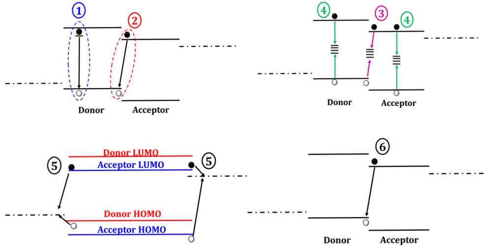
Fig. 3. 6. Recombination pathways in a BHJ: (1) Excitonic, (2) Geminate, (3) D/A interface trap-assisted, (4) Trap-assisted inside the domains, (5) contact, and (6) Band-to-band recombination.
