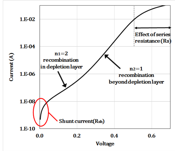
Fig. 2. 4. Dark IV of a silicon PN junction. For this diode: I_{01}=4\times 10^{-9} A, n_1=2 , I_{02}=4\times 10^{-11} A, n_2=1 , R_{sh}=10^7\Omega and R_s=1\Omega for a device area of 0.1\text{ cm}^2 50 .
