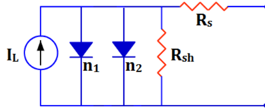
Fig. 2. 2. Double-diode equivalent circuit of a solar cell. n_1 and n_2 are ideality factors of the diodes 50 .
