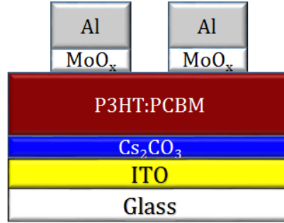
Fig. 5. 2. Reference n-i-p cell with Cs_2CO_3 as ETL.
