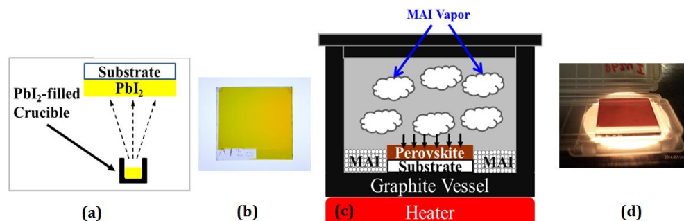
Fig. 6.14. Vapor-assisted perovskite growth: (a) Thermal evaporation of PbI_2 resulting in (b) a transparent yellow film, (c) exposure of the PbI_2 film to MAI vapors in an enclosed heated graphite vessel leads to the formation of (d) dark brown methyl-ammonium lead iodide.
