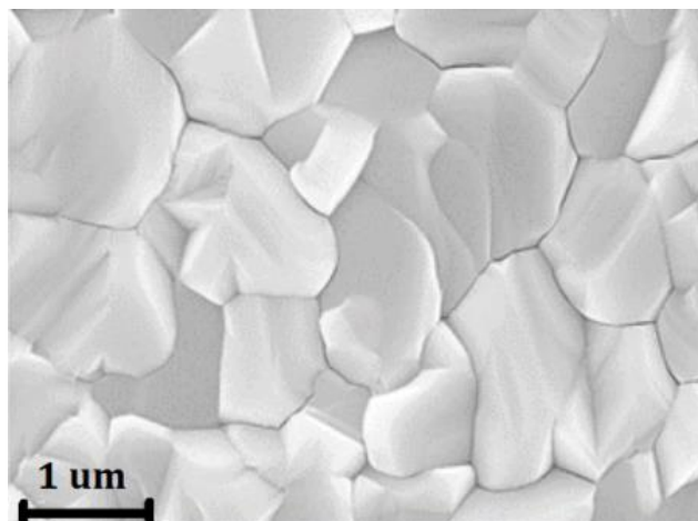
Fig. 6. 15. SEM micrograph of perovskite film deposited by vapor-assisted growth on top of TiO 2 -coated FTO substrate. A compact arrangement of large grains is observed.
