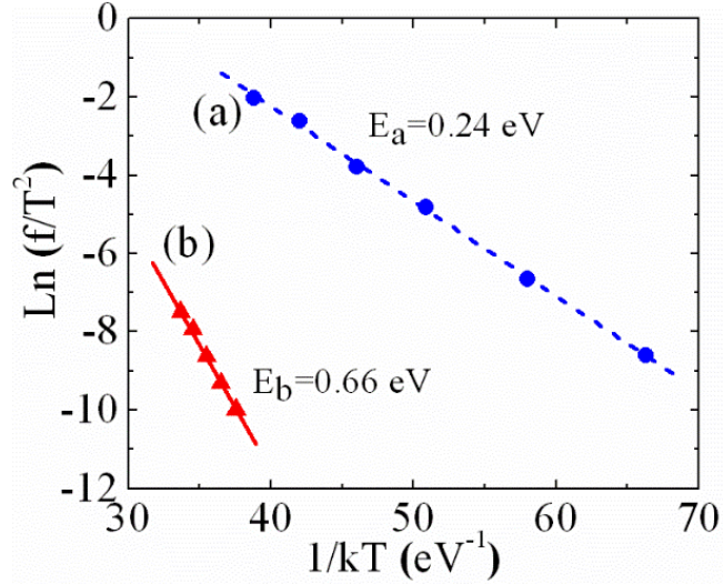
Fig. 6. 22. Two defect bands are obtained from the Arrhenius diagram: (a) 0.24 eV, and (b) 0.66 eV below the conduction band edge.
