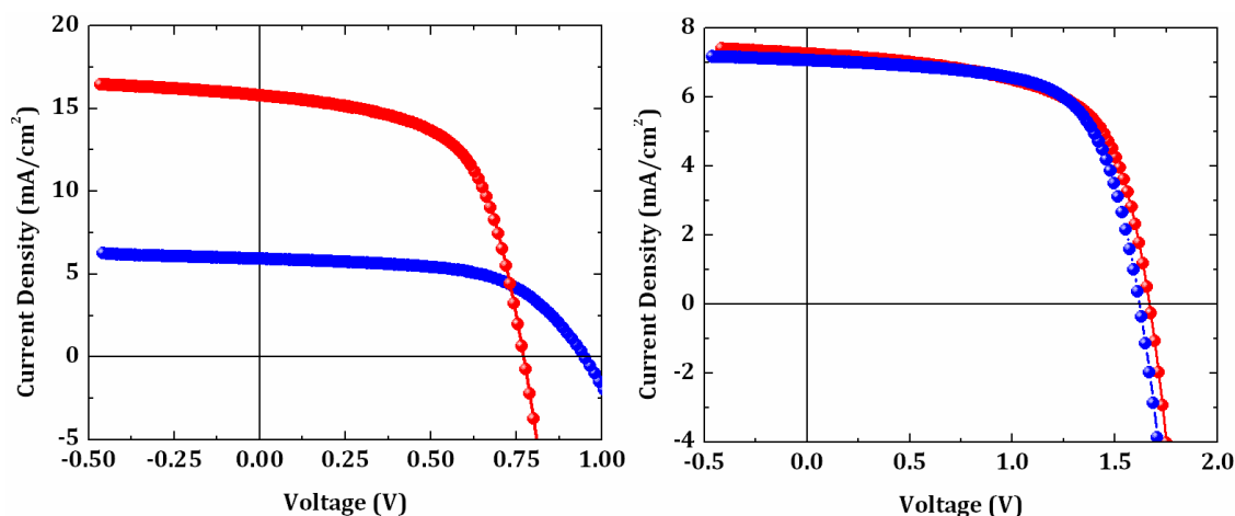
Fig. 5. 12. Left-JV characteristics of single junction p-i-n PTB7:PCBM70 (red) and a -(Si,C):H (blue) cells. Right- JV characteristics of tandem cells of Fig. 5. 11 with MoO x (red) and PEDOT:PSS (blue) interlayers.
